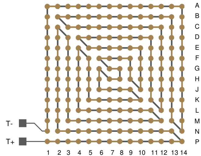
AFTER MOUNTING
